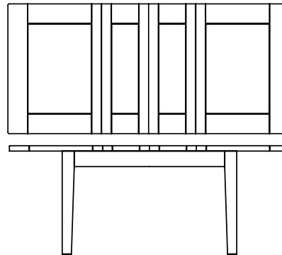
4' 6" EXTENDING TABLE (2 LEAF) H 778 W: 1320-1984 D: 915
