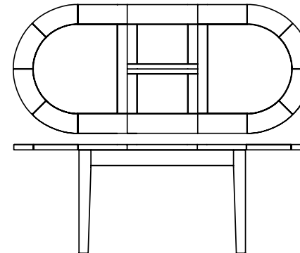
LARGE D-END EXTENDING TABLE H 778 W: 1615-2115 D: 915
